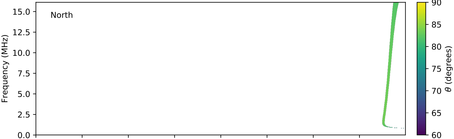
expres_cassini_jupiter_europa_isaac_lossc-wid1deg_3kev_20020503_v01.cdf
