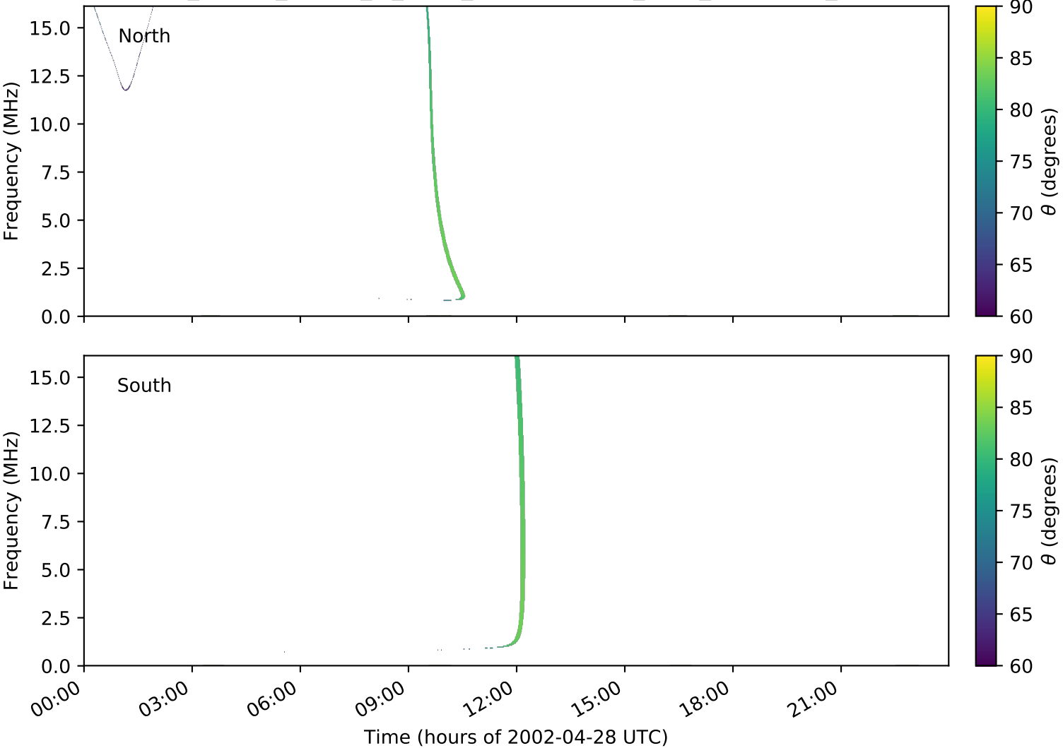
expres_cassini_jupiter_io_isaac_lossc-wid1deg_3kev_20020428_v01.cdf
