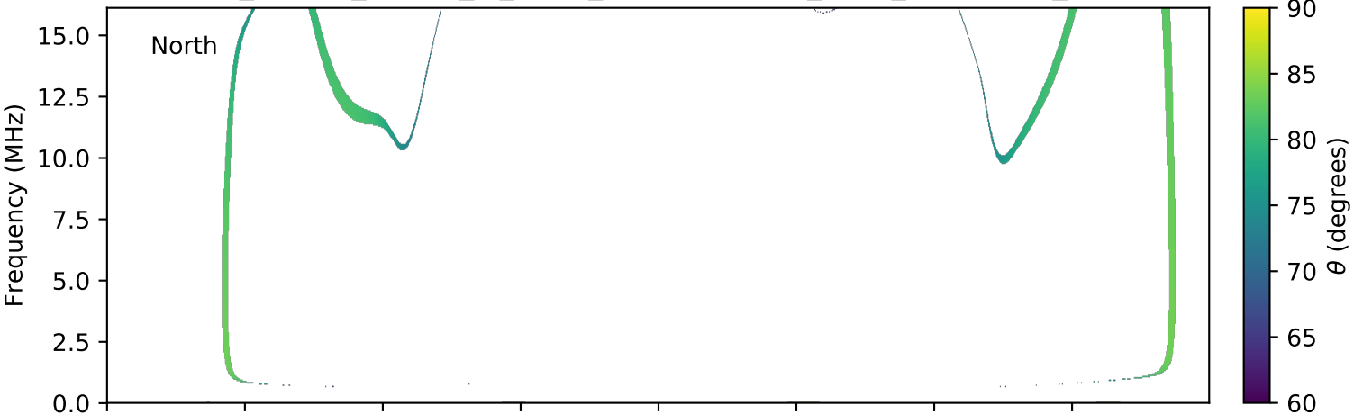
expres_cassini_jupiter_io_isaac_lossc-wid1deg_3kev_20020424_v01.cdf
