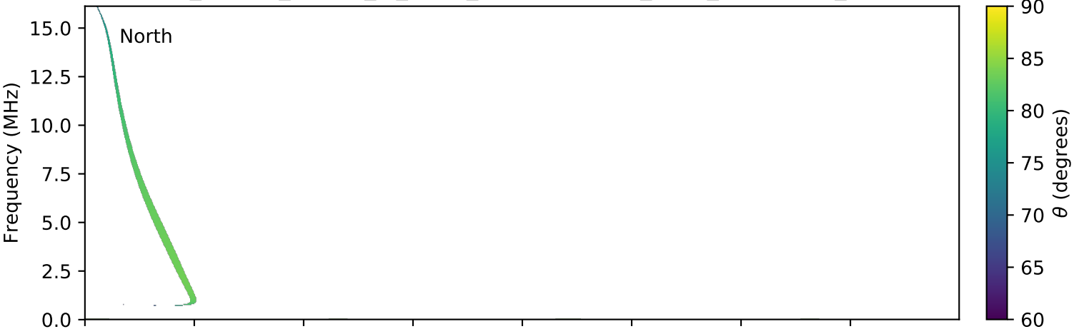
expres_cassini_jupiter_io_isaac_lossc-wid1deg_3kev_20020423_v01.cdf
