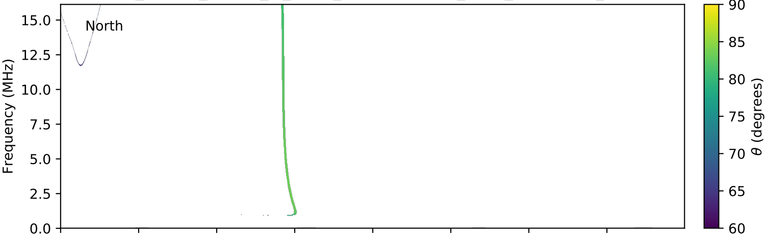
expres_cassini_jupiter_io_isaac_lossc-wid1deg_3kev_20020421_v01.cdf
