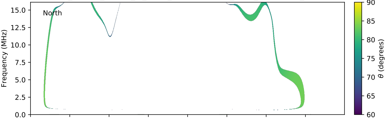
expres_cassini_jupiter_io_isaac_lossc-wid1deg_3kev_20020417_v01.cdf
