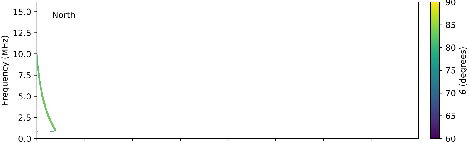
expres_cassini_jupiter_io_isaac_lossc-wid1deg_3kev_20020416_v01.cdf
