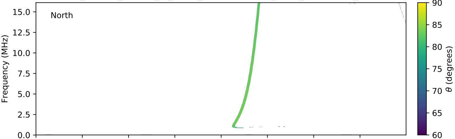
expres_cassini_jupiter_io_isaac_lossc-wid1deg_3kev_20020413_v01.cdf
