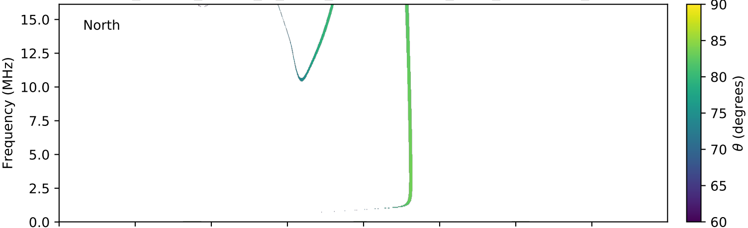
expres_cassini_jupiter_io_isaac_lossc-wid1deg_3kev_20020412_v01.cdf
