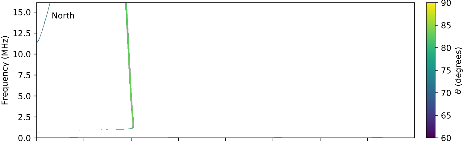
expres_cassini_jupiter_io_isaac_lossc-wid1deg_3kev_20020407_v01.cdf
