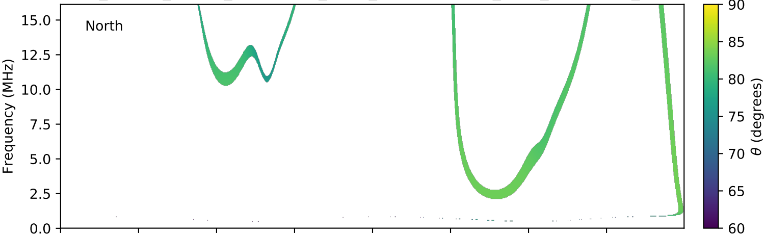
expres_cassini_jupiter_ganymede_isaac_lossc-wid1deg_3kev_20020429_v01.cdf
