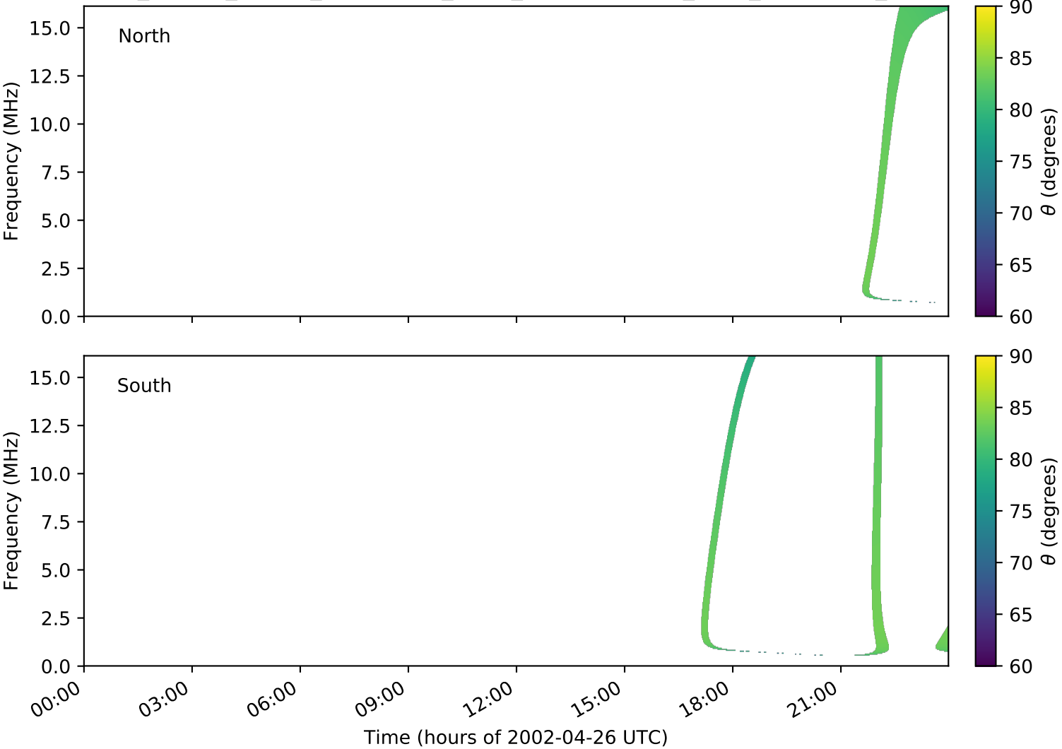
expres_cassini_jupiter_ganymede_isaac_lossc-wid1deg_3kev_20020426_v01.cdf
