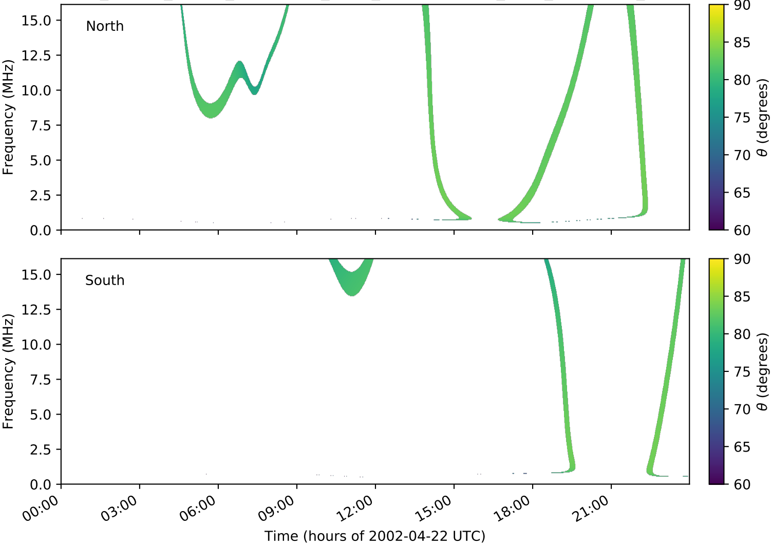
expres_cassini_jupiter_ganymede_isaac_lossc-wid1deg_3kev_20020422_v01.cdf
