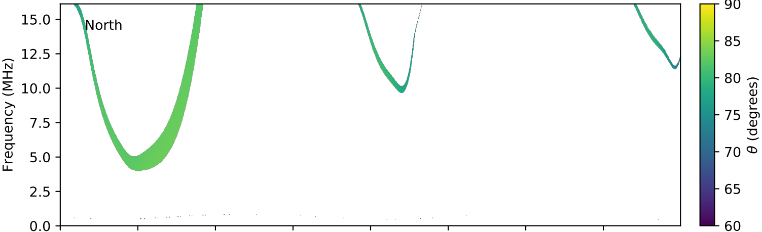
expres_cassini_jupiter_ganymede_isaac_lossc-wid1deg_3kev_20020420_v01.cdf
