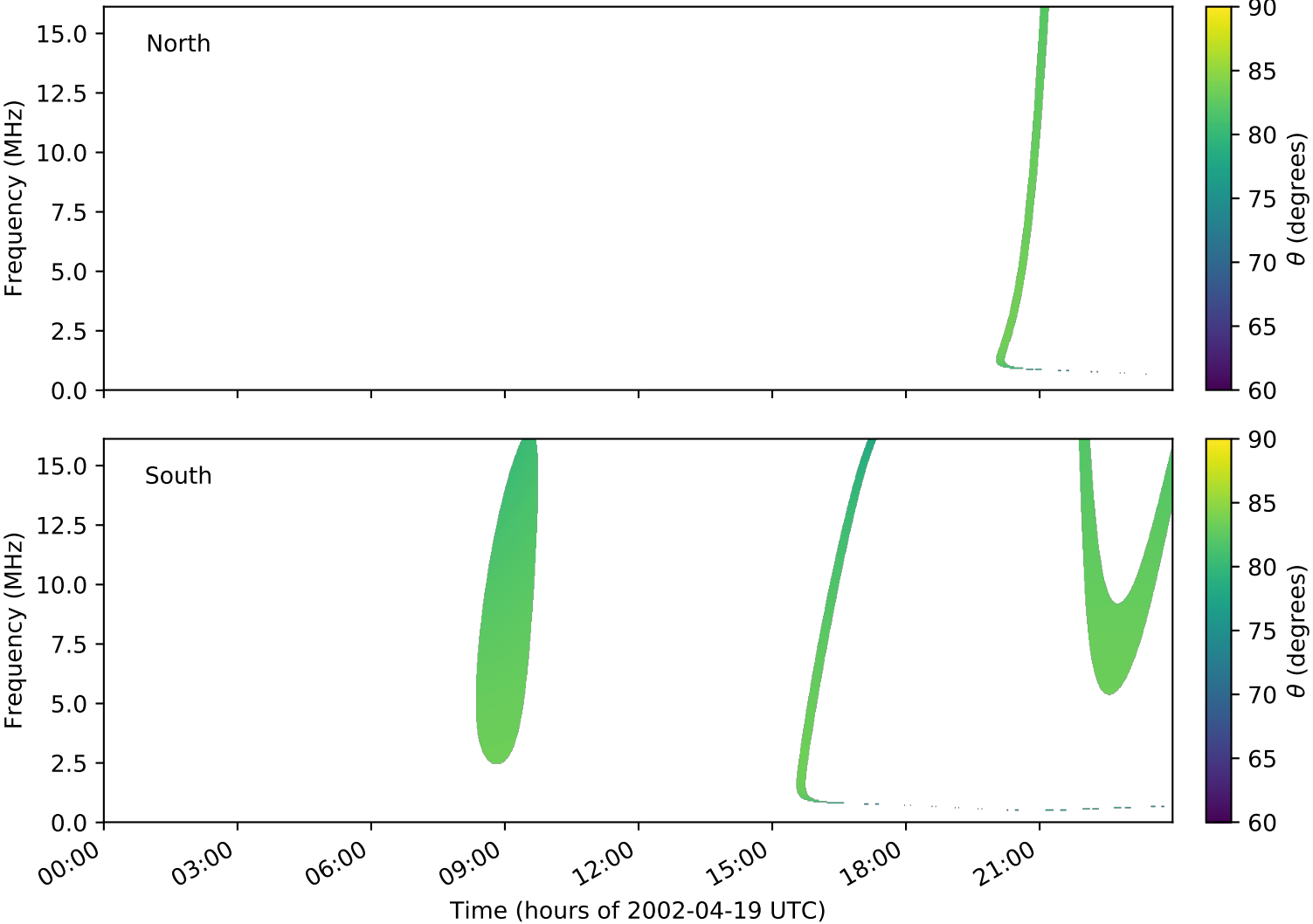
expres_cassini_jupiter_ganymede_isaac_lossc-wid1deg_3kev_20020419_v01.cdf
