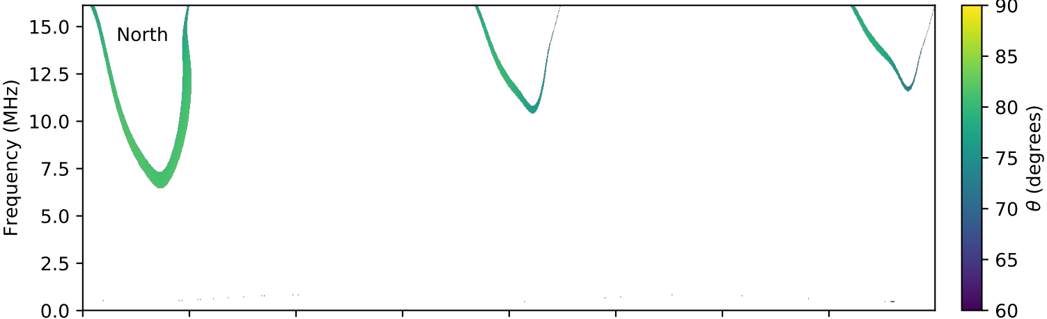
expres_cassini_jupiter_ganymede_isaac_lossc-wid1deg_3kev_20020413_v01.cdf
