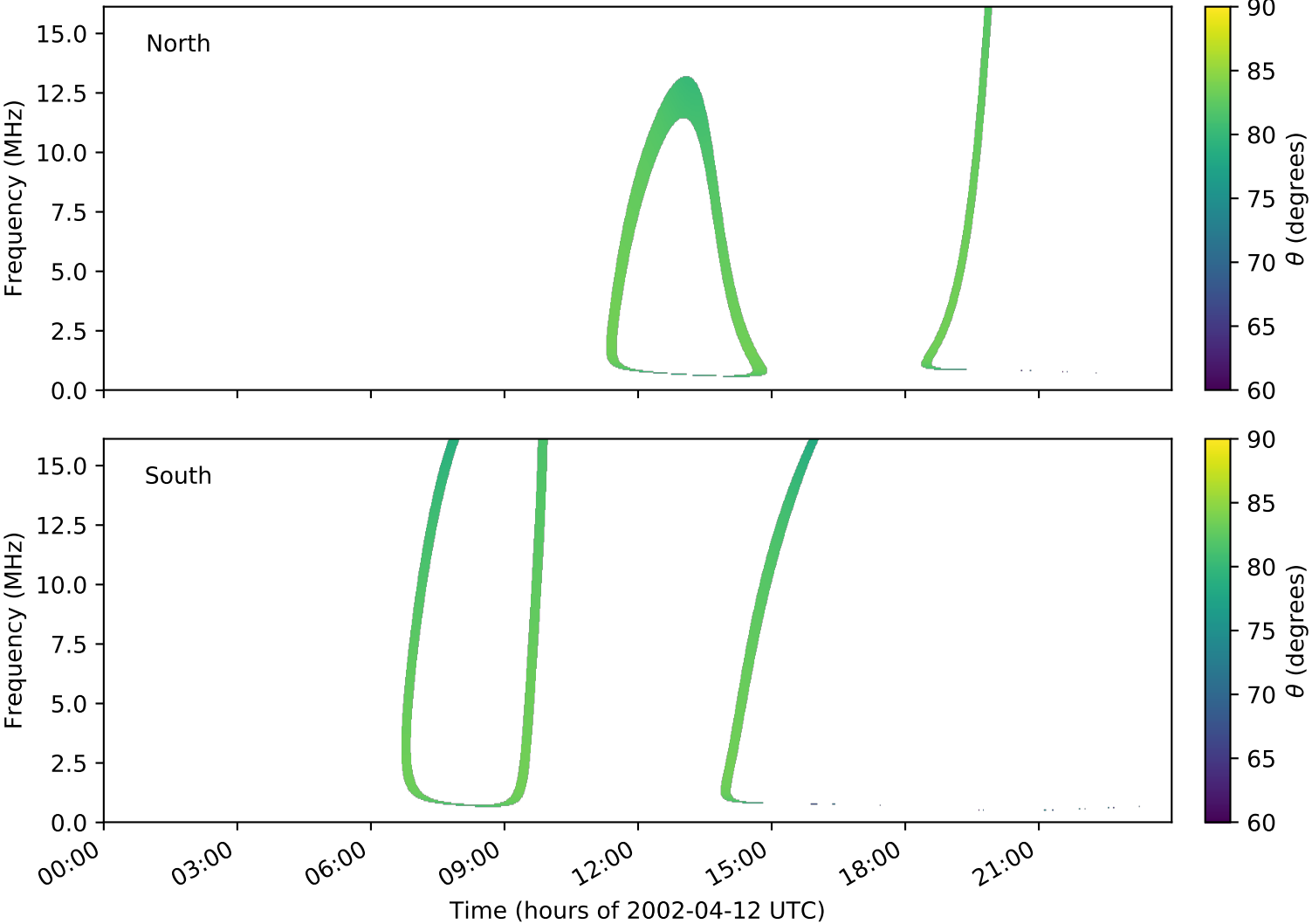
expres_cassini_jupiter_ganymede_isaac_lossc-wid1deg_3kev_20020412_v01.cdf
