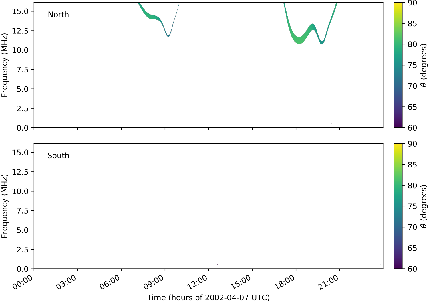
expres_cassini_jupiter_ganymede_isaac_lossc-wid1deg_3kev_20020407_v01.cdf
