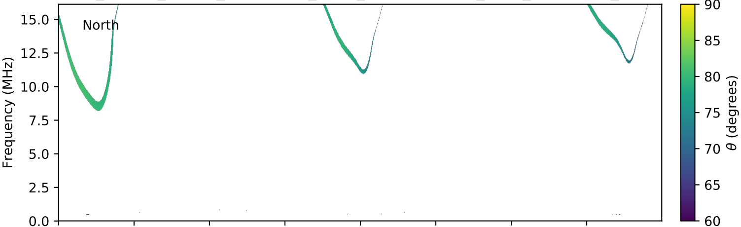
expres_cassini_jupiter_ganymede_isaac_lossc-wid1deg_3kev_20020406_v01.cdf
