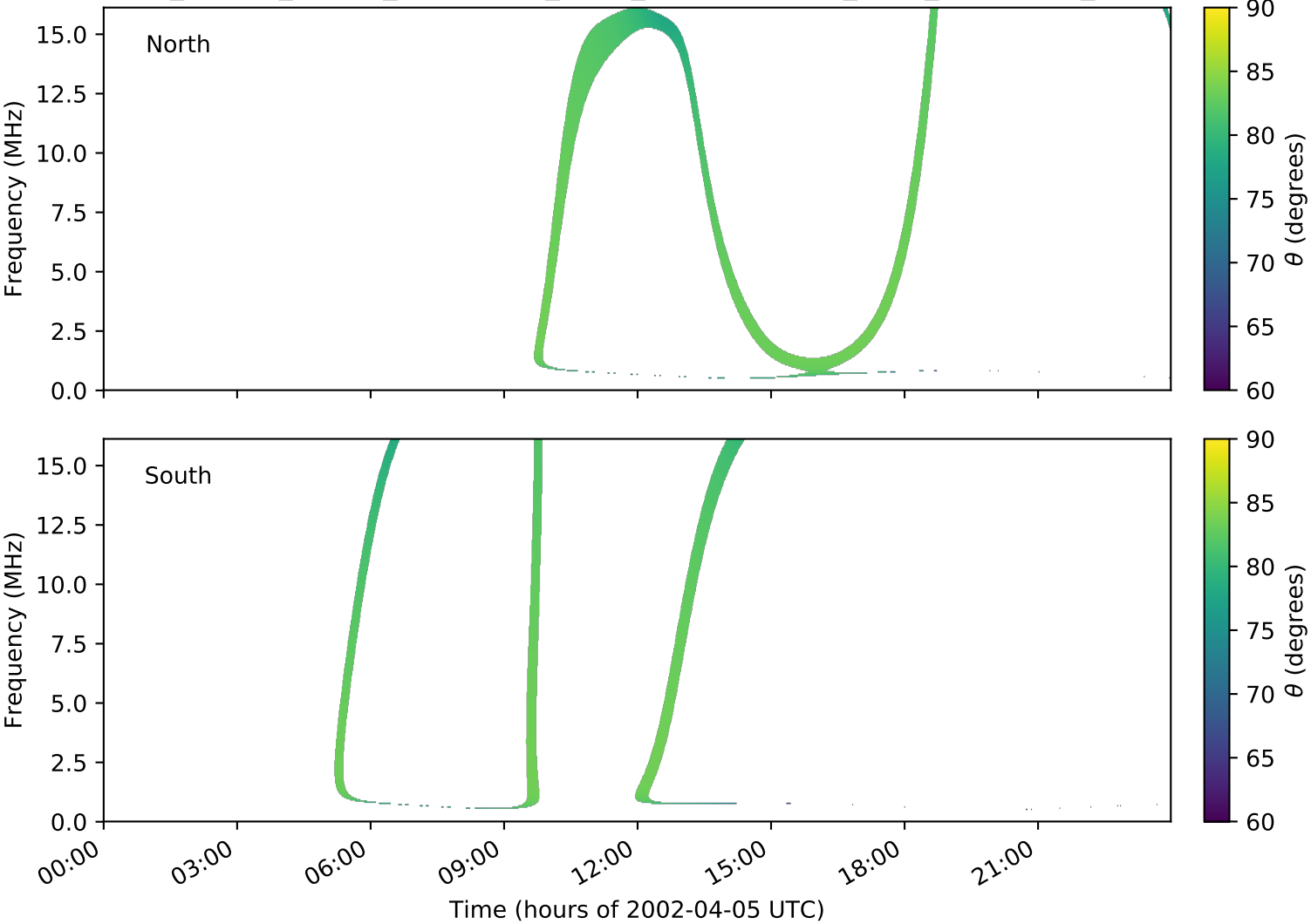
expres_cassini_jupiter_ganymede_isaac_lossc-wid1deg_3kev_20020405_v01.cdf
