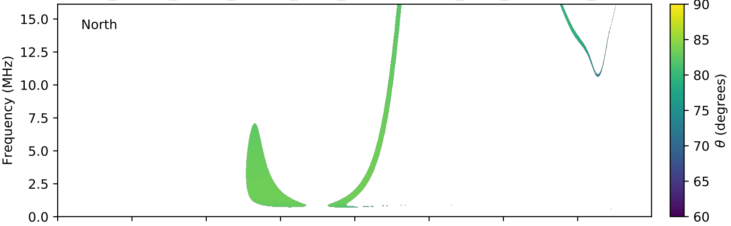
expres_cassini_jupiter_europa_isaac_lossc-wid1deg_3kev_20020430_v01.cdf
