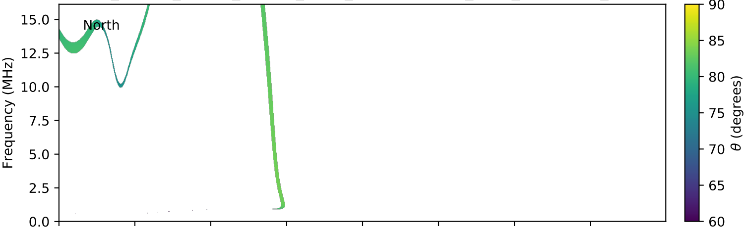
expres_cassini_jupiter_europa_isaac_lossc-wid1deg_3kev_20020428_v01.cdf
