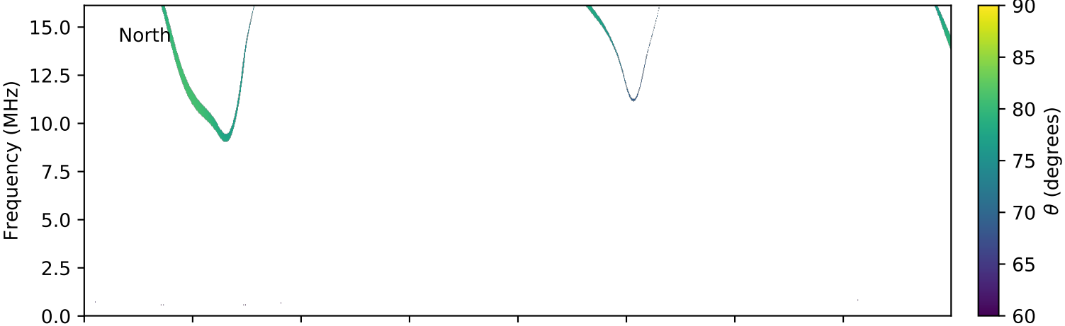
expres_cassini_jupiter_europa_isaac_lossc-wid1deg_3kev_20020427_v01.cdf
