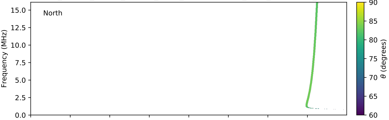
expres_cassini_jupiter_europa_isaac_lossc-wid1deg_3kev_20020426_v01.cdf
