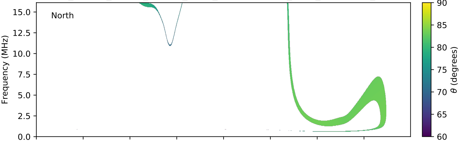
expres_cassini_jupiter_europa_isaac_lossc-wid1deg_3kev_20020424_v01.cdf
