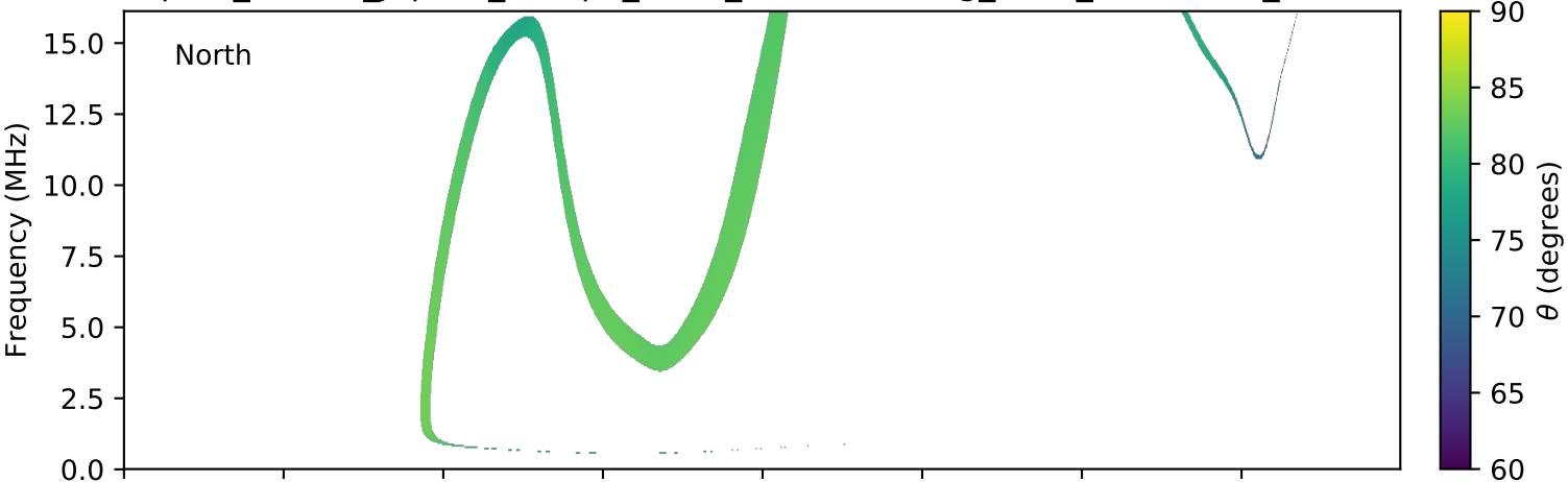
expres_cassini_jupiter_europa_isaac_lossc-wid1deg_3kev_20020423_v01.cdf
