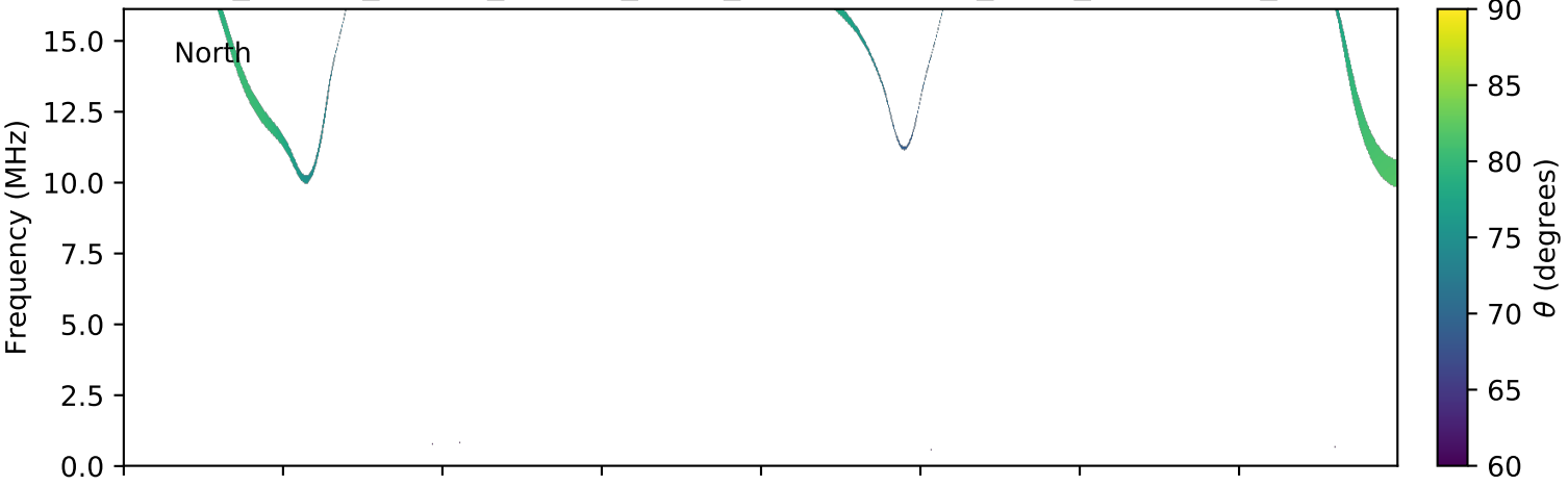
expres_cassini_jupiter_europa_isaac_lossc-wid1deg_3kev_20020420_v01.cdf
