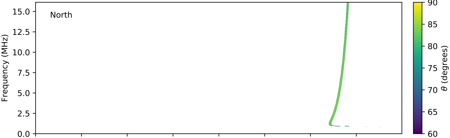
expres_cassini_jupiter_europa_isaac_lossc-wid1deg_3kev_20020419_v01.cdf
