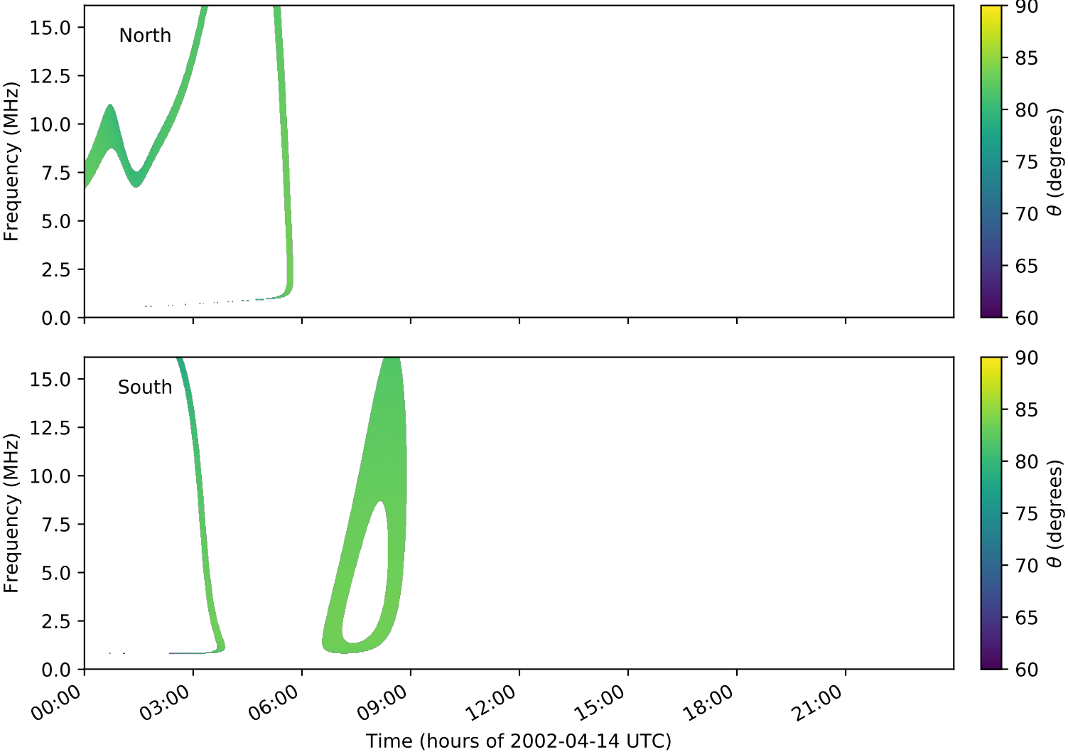
expres_cassini_jupiter_europa_isaac_lossc-wid1deg_3kev_20020414_v01.cdf
