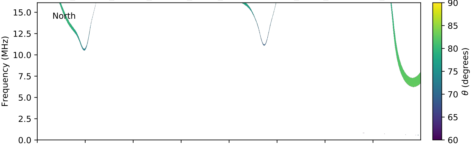
expres_cassini_jupiter_europa_isaac_lossc-wid1deg_3kev_20020413_v01.cdf
