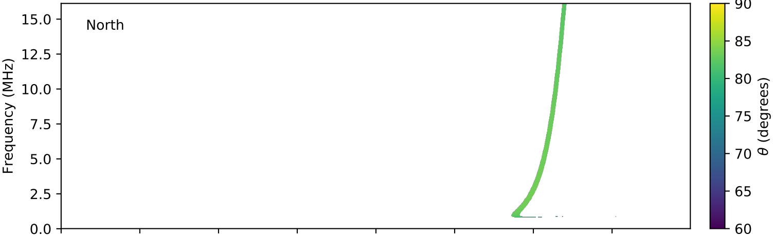
expres_cassini_jupiter_europa_isaac_lossc-wid1deg_3kev_20020412_v01.cdf
