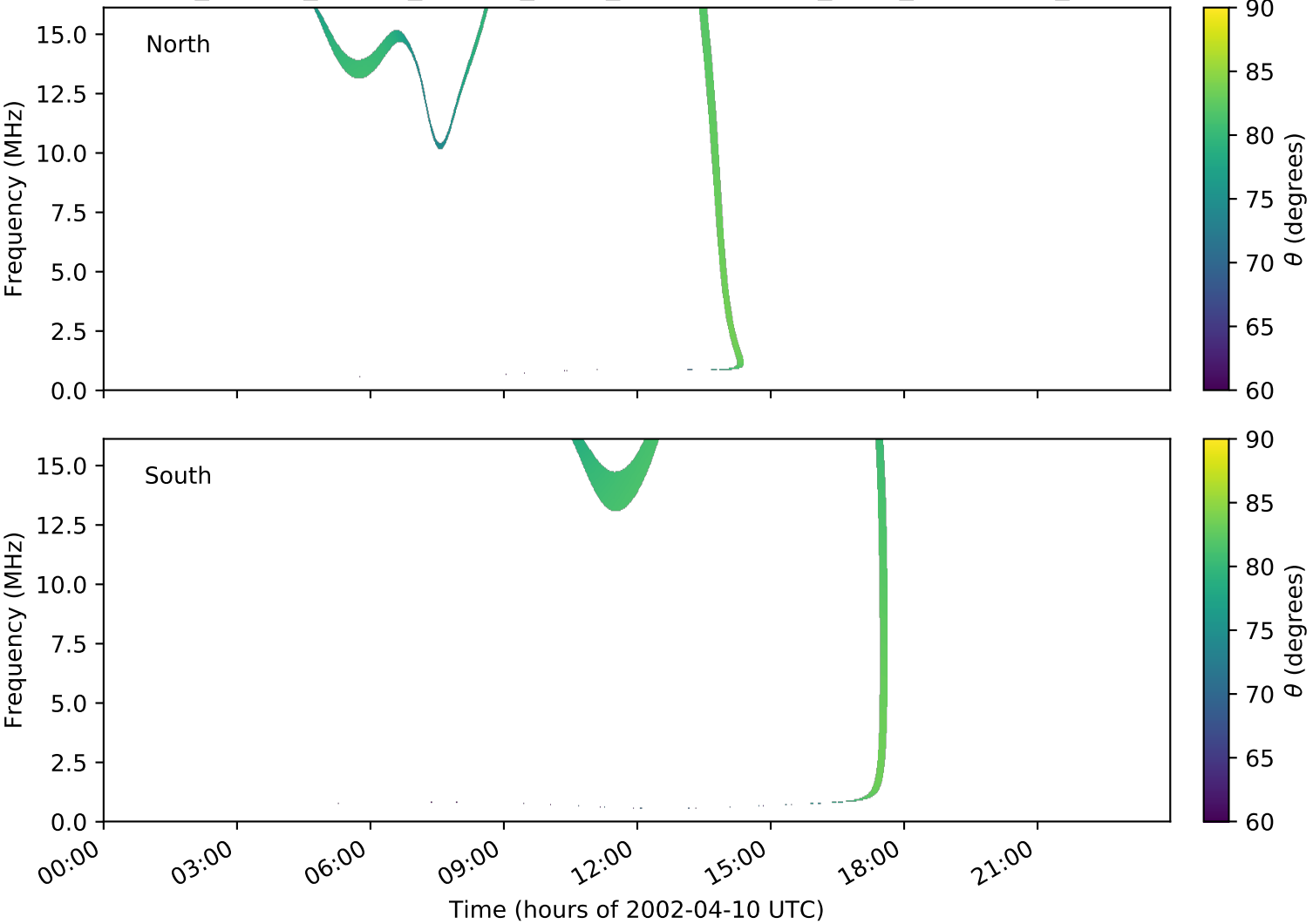
expres_cassini_jupiter_europa_isaac_lossc-wid1deg_3kev_20020410_v01.cdf
