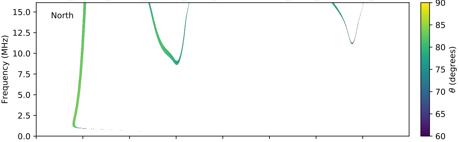
expres_cassini_jupiter_europa_isaac_lossc-wid1deg_3kev_20020409_v01.cdf
