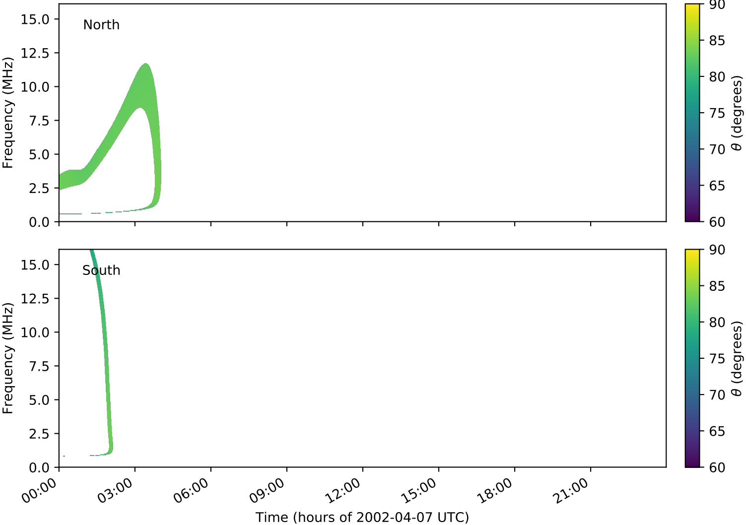
expres_cassini_jupiter_europa_isaac_lossc-wid1deg_3kev_20020407_v01.cdf
