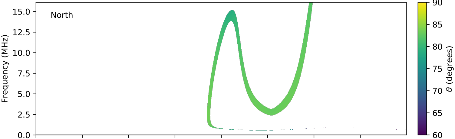
expres_cassini_jupiter_europa_isaac_lossc-wid1deg_3kev_20020405_v01.cdf
