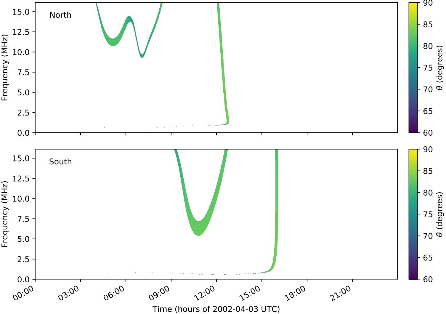
expres_cassini_jupiter_europa_isaac_lossc-wid1deg_3kev_20020403_v01.cdf
