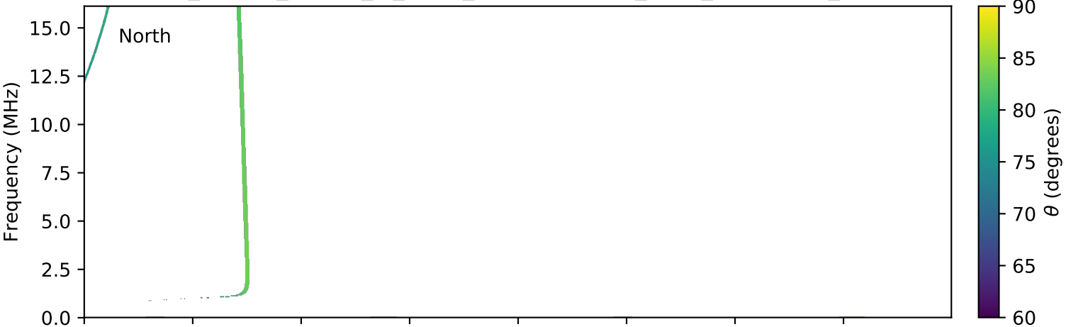
expres_cassini_jupiter_io_isaac_lossc-wid1deg_3kev_20020331_v01.cdf
