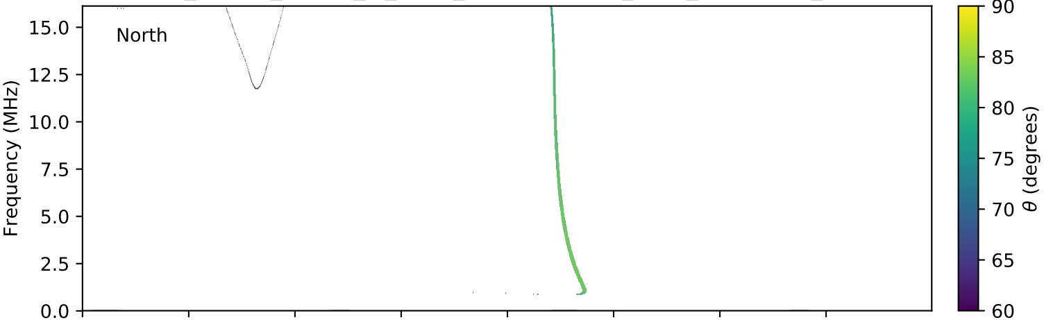
expres_cassini_jupiter_io_isaac_lossc-wid1deg_3kev_20020327_v01.cdf
