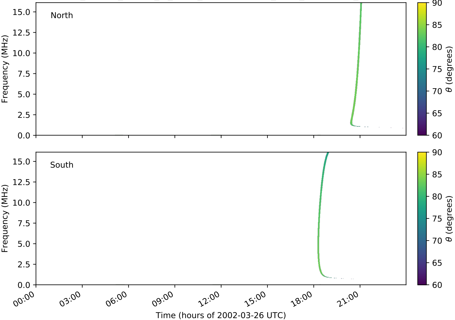
expres_cassini_jupiter_io_isaac_lossc-wid1deg_3kev_20020326_v01.cdf
