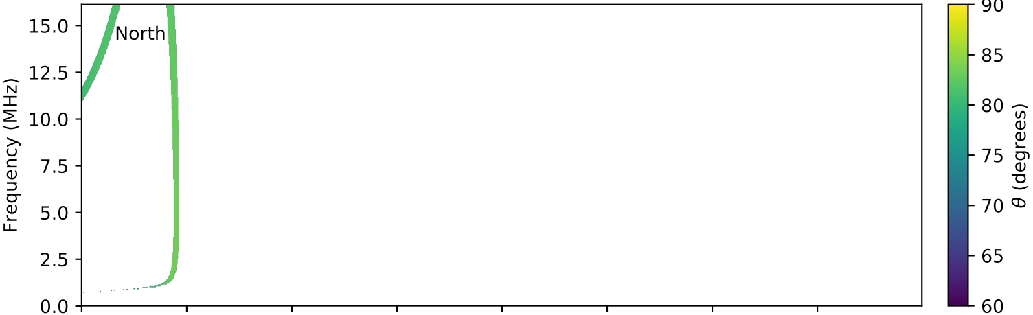
expres_cassini_jupiter_io_isaac_lossc-wid1deg_3kev_20020324_v01.cdf
