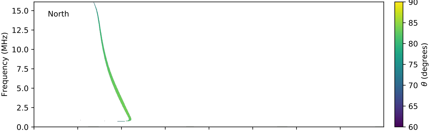
expres_cassini_jupiter_io_isaac_lossc-wid1deg_3kev_20020322_v01.cdf
