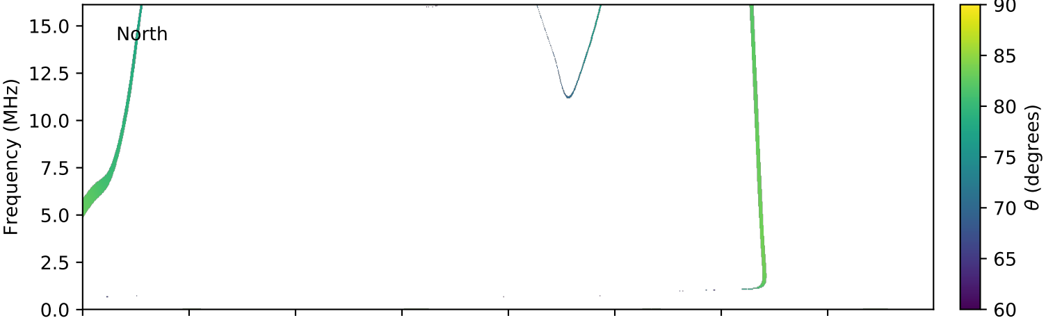
expres_cassini_jupiter_io_isaac_lossc-wid1deg_3kev_20020318_v01.cdf
