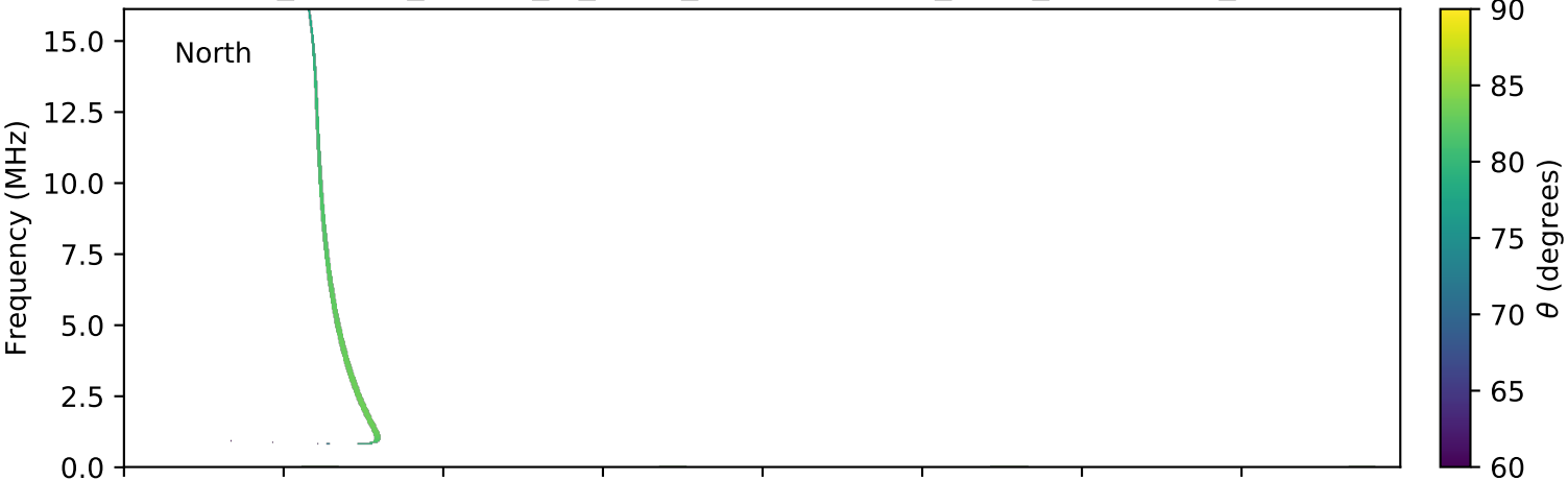
expres_cassini_jupiter_io_isaac_lossc-wid1deg_3kev_20020315_v01.cdf
