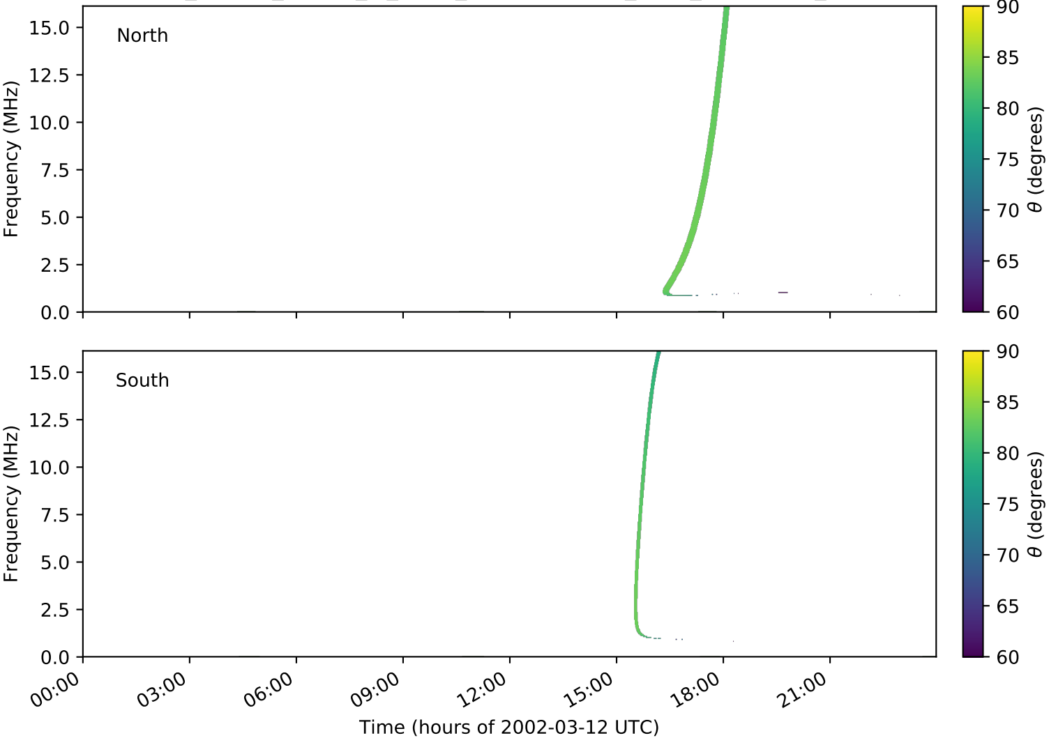
expres_cassini_jupiter_io_isaac_lossc-wid1deg_3kev_20020312_v01.cdf
