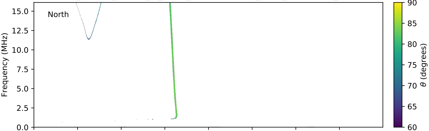
expres_cassini_jupiter_io_isaac_lossc-wid1deg_3kev_20020306_v01.cdf
