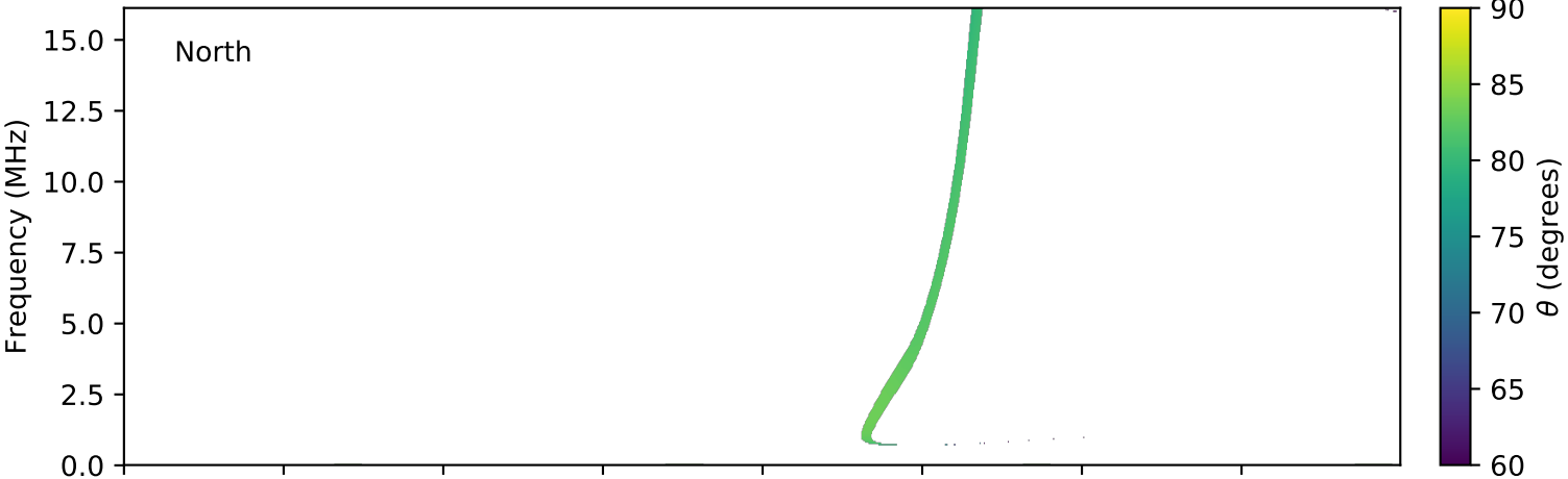
expres_cassini_jupiter_io_isaac_lossc-wid1deg_3kev_20020305_v01.cdf
