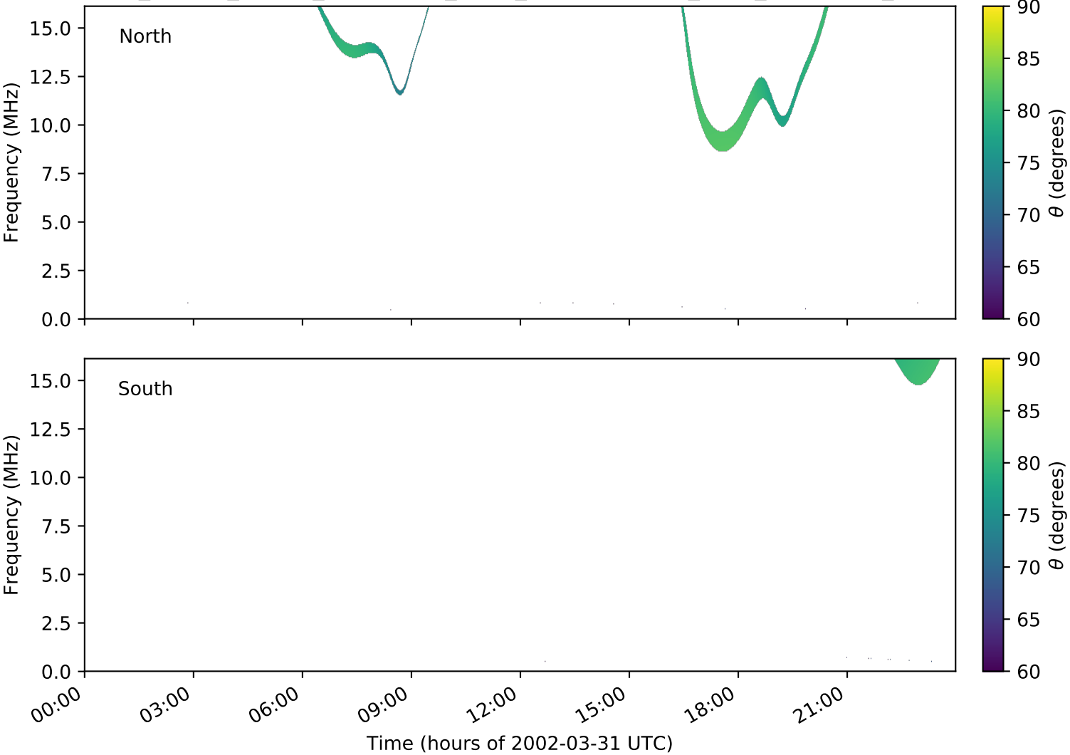
expres_cassini_jupiter_ganymede_isaac_lossc-wid1deg_3kev_20020331_v01.cdf
