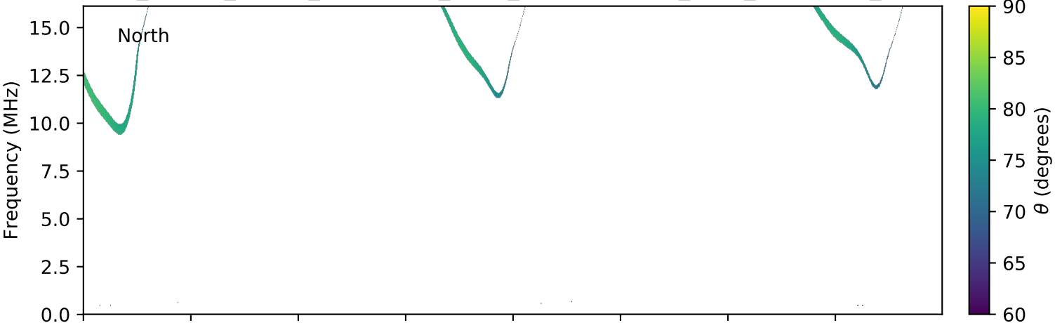
expres_cassini_jupiter_ganymede_isaac_lossc-wid1deg_3kev_20020330_v01.cdf
