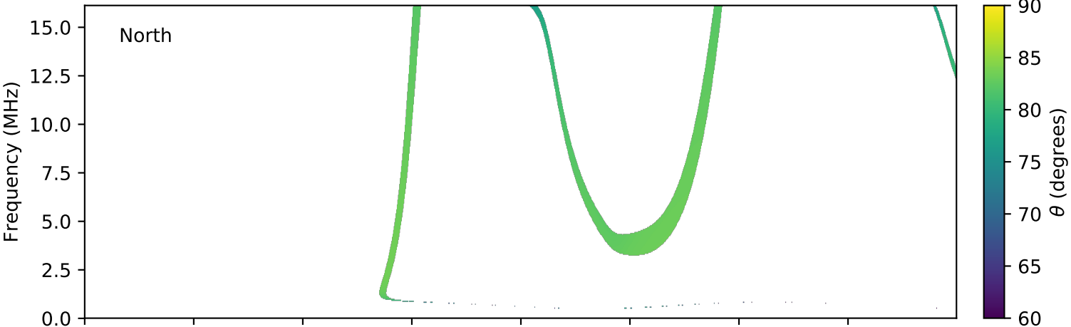
expres_cassini_jupiter_ganymede_isaac_lossc-wid1deg_3kev_20020329_v01.cdf
