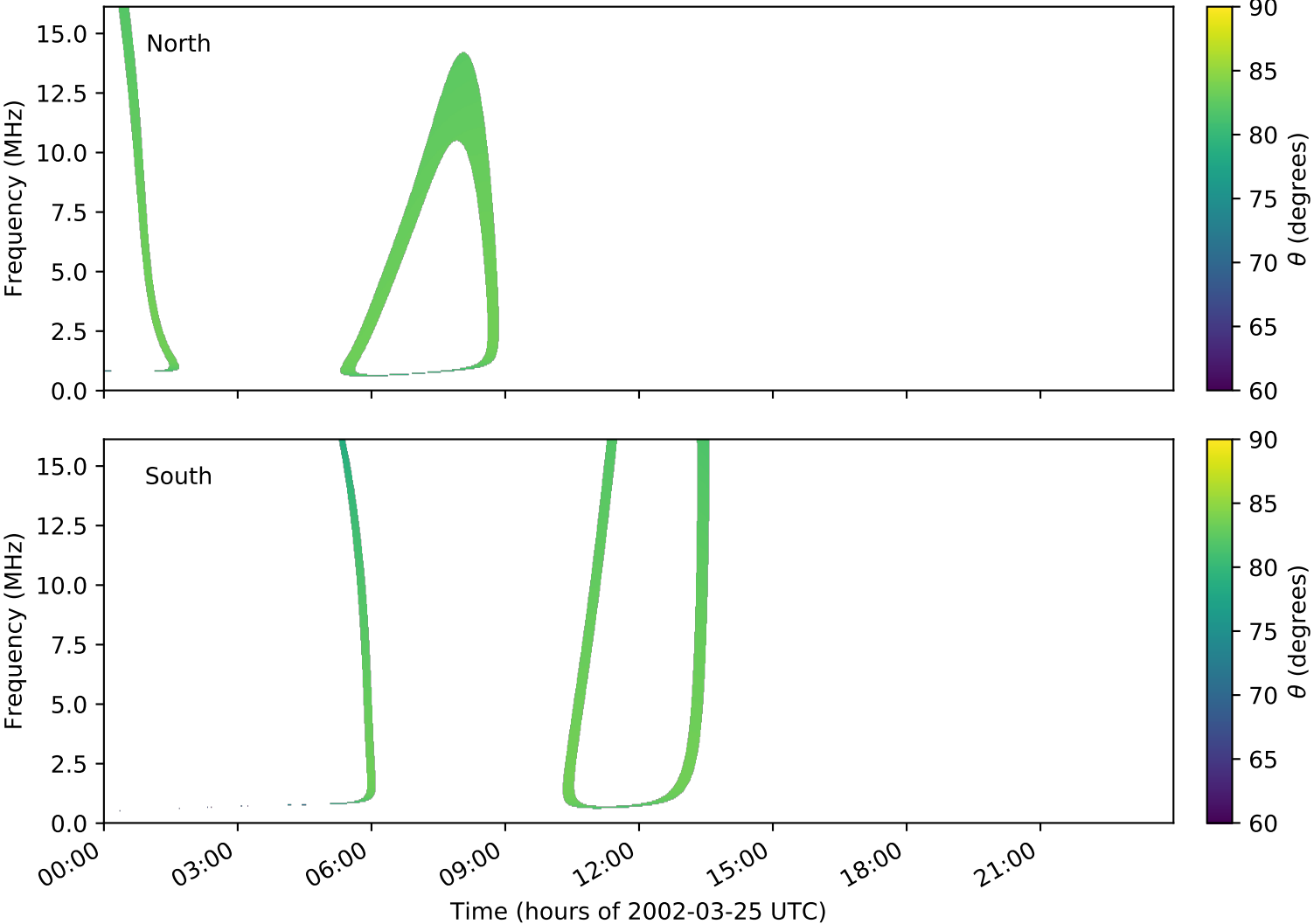
expres_cassini_jupiter_ganymede_isaac_lossc-wid1deg_3kev_20020325_v01.cdf
